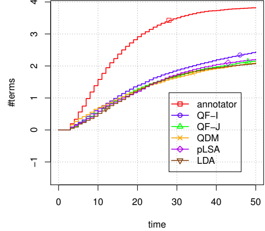
Figure 3: Number of feedback terms selected over time on facets generated by different models, based on annotator feedback.
