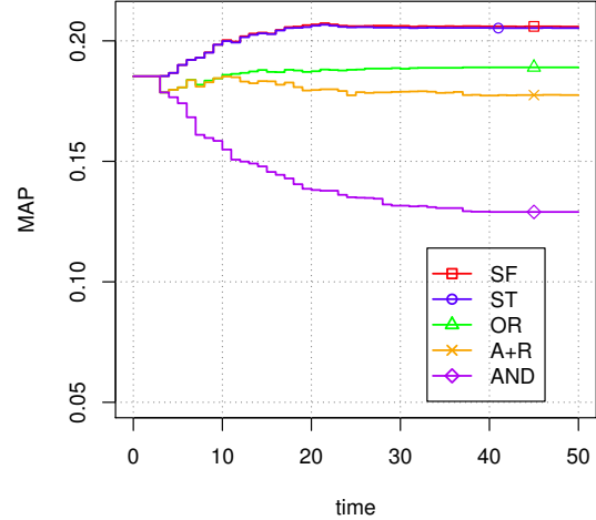
Figure 6: MAP change over time for different feedback models, based on annotator facets and annotator feedback.
